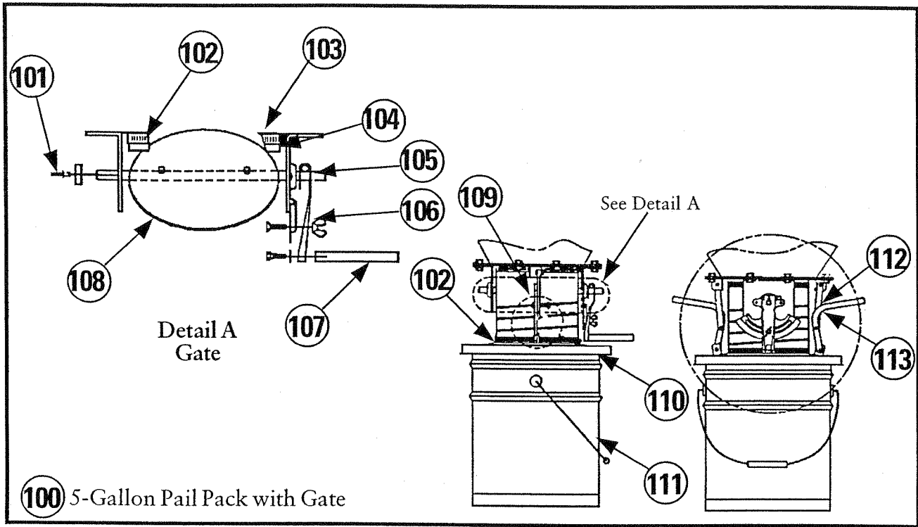
Parts Drawing 9 5-Gallon Pail Pack
