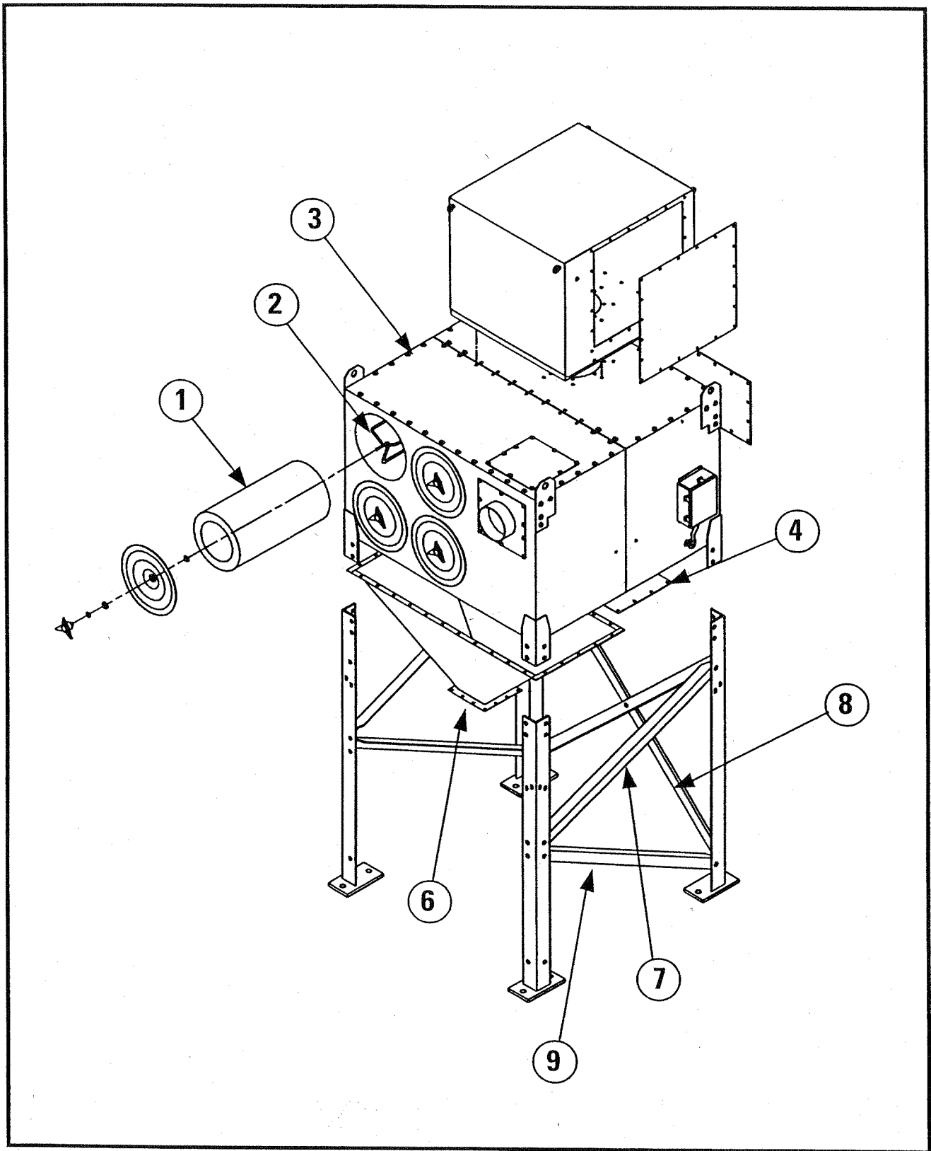
Parts Drawing 1 Empire Dust Collector (Model EM 2-4)
