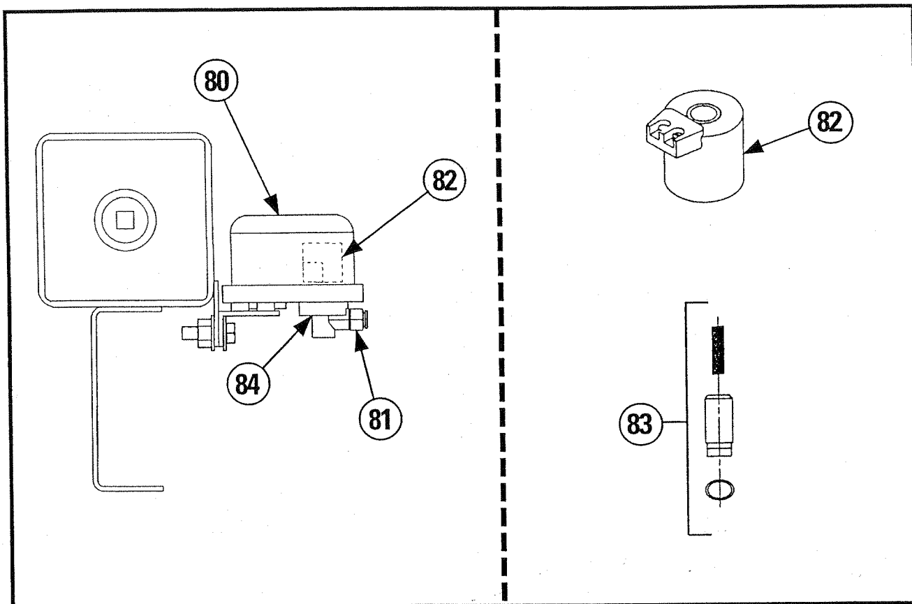
Parts Drawing 8 Solenoid Pack Assembly NEMA 4 EM 2-4
