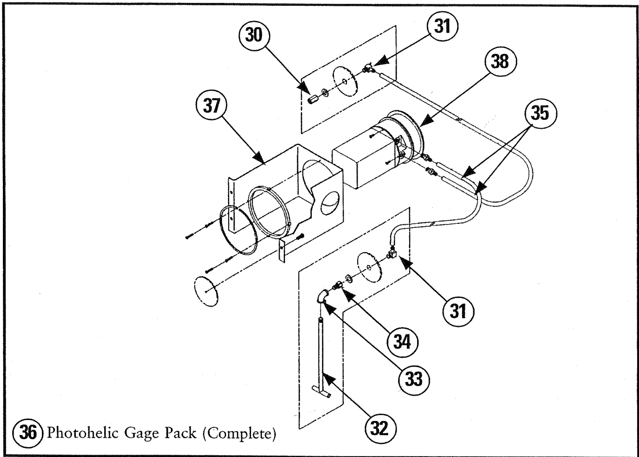
Parts Drawing 3 Photohelic Pack
