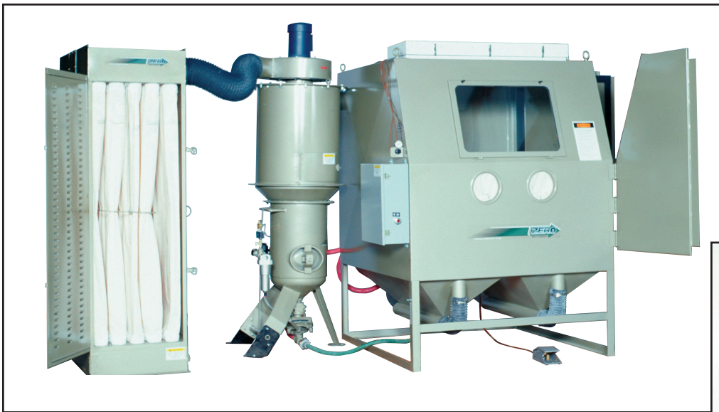
Model BNP-720 with 900 CFM Reclaimer and Dry Filter Dust Collector
